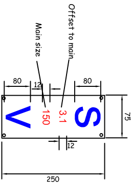
EXAMPLE OF MARKER PLATE
